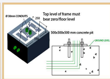
FOUNDATION FRAME
