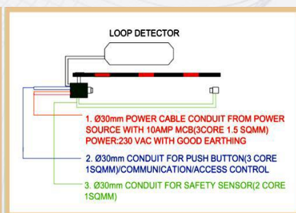
ELECTRICAL PROVISIONS
