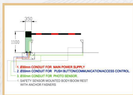
CIVIL PROVISIONS
